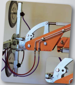
The lifting head has two settings, adjusted by means of two holes for the locking bolt. The lifting head can therefore be adjusted to tilt more towards the ceiling or floor.
