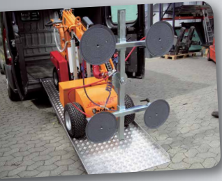
The Smartlift is easily transported in a van or on a trailer
